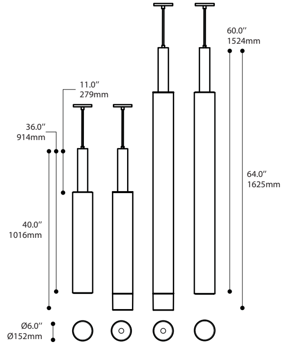
OPTIONAL DOWNLIGHT MODULE 11W LED COB with 20° or 40° beam angle
