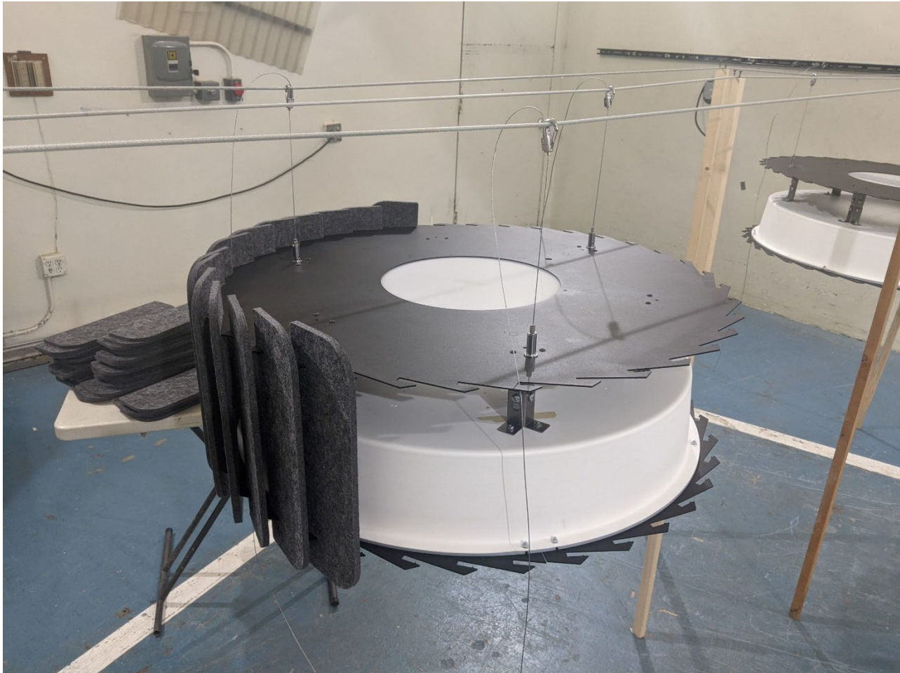
Figure 5 – Specimen fins partially installed to hubs
